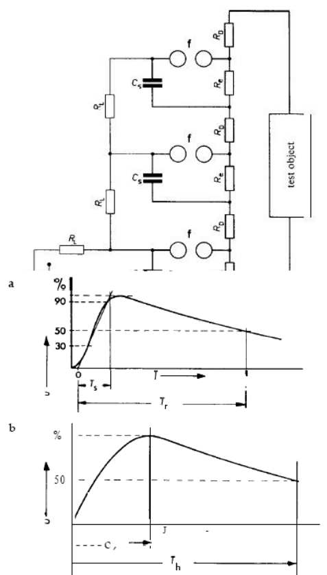
Fig. 4 Standardized test voltages a Lightning impulse voltage 1.2/50 Front time: T_s = 1.2 \pm 0.36 \mu s Time of half value: T_r = 50 \pm 10 \mu s b Switching impulse voltage 250/2500 Front time: T_{fr} = 250 \pm 50 \mu s Time of half value: T_h = 2500 \pm 1500 \mu s
